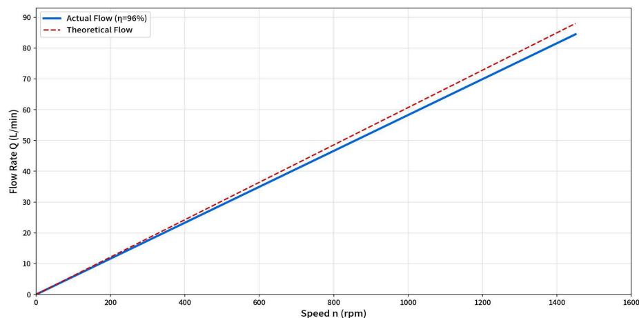
3-Cylinder Plunger Pump - Flow vs. Speed Characteristic
