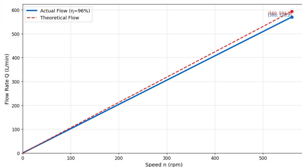
6-Cylinder Plunger Pump - Flow vs. Speed Characteristic
